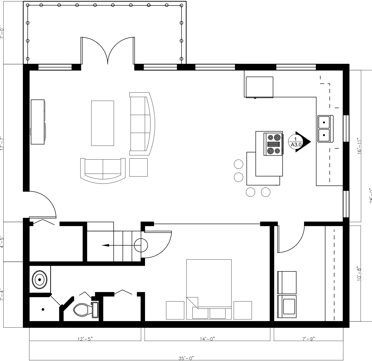
FLOOR PLAN
